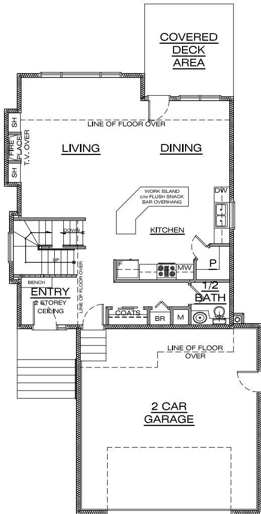
MAIN FLOOR 916 sq. ft.
