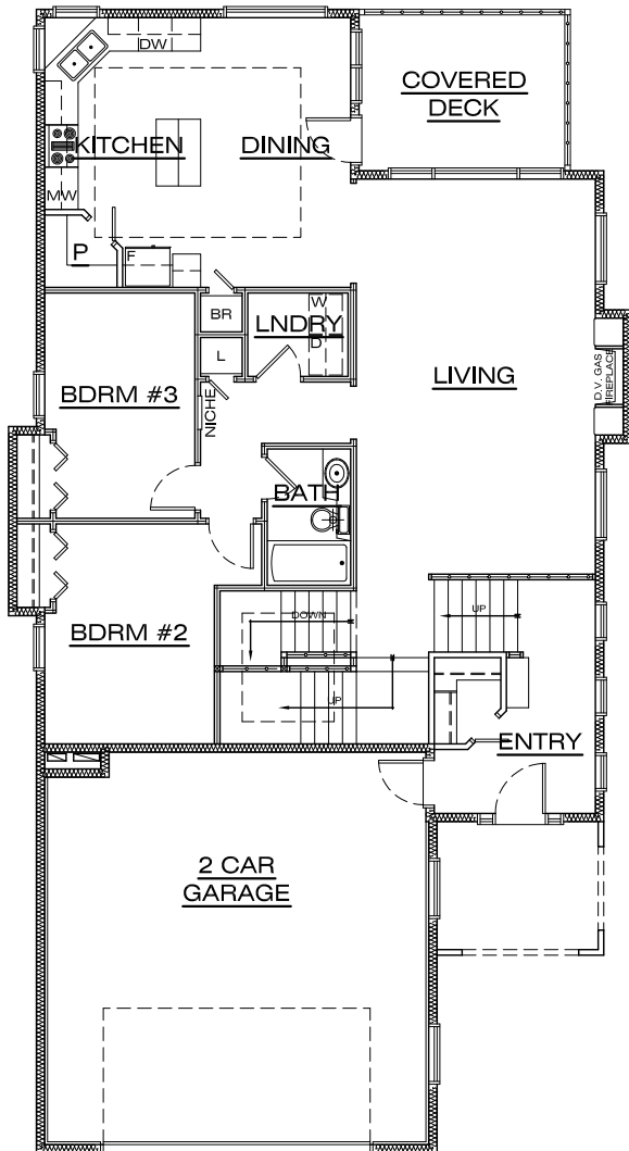
MAIN FLOOR 1449 sq. ft.
